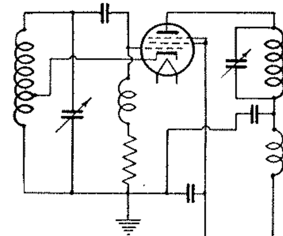
Fig. 5. Electron-Coupled Tri-Tet Oscillator
