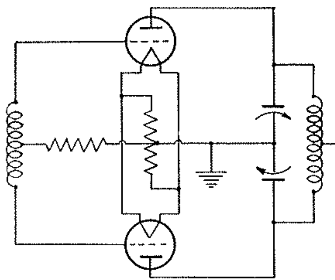
Fig. 4. Push-Pull Oscillator
